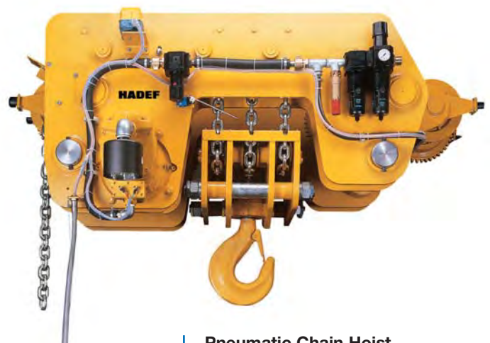
Pneumatic Chain Hoist Type 29/06 APP with pneumatic trolley capacity 30 t / 6 chain falls offshore-design
