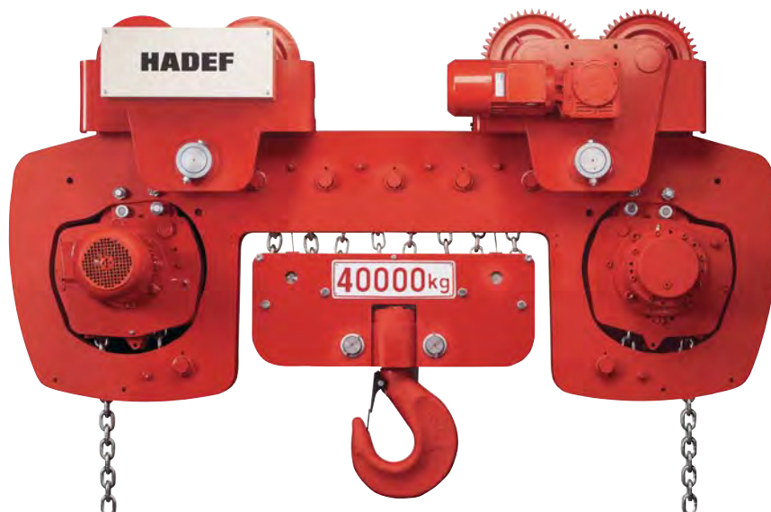
Type 28/06 EE capacity 40 t / 8 chain falls
