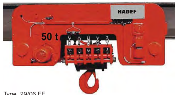
Type 29/06 EE capacity 50 t 10 chain falls
